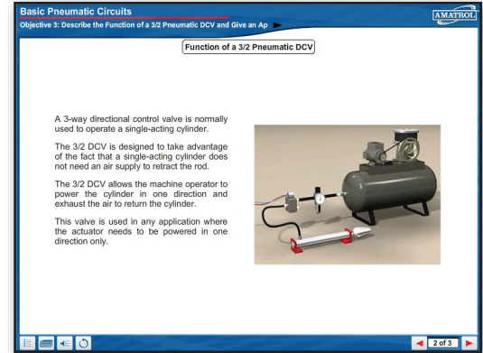
3/2 DCV in 990-PN1's Multimedia
