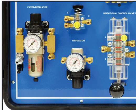
Air Filter on the 990-PN1
