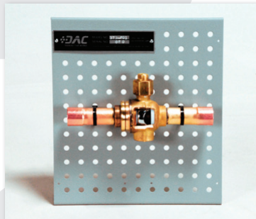
373-501 ACR Steel Ball Valve
